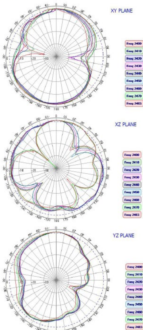
WIFI Antenna
